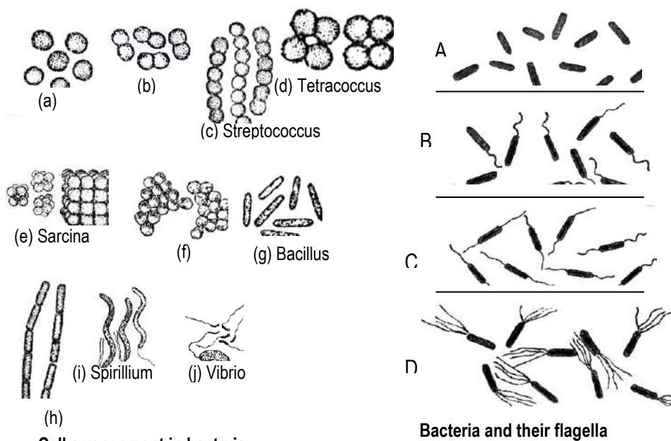
Cell arrangement in bacteria
