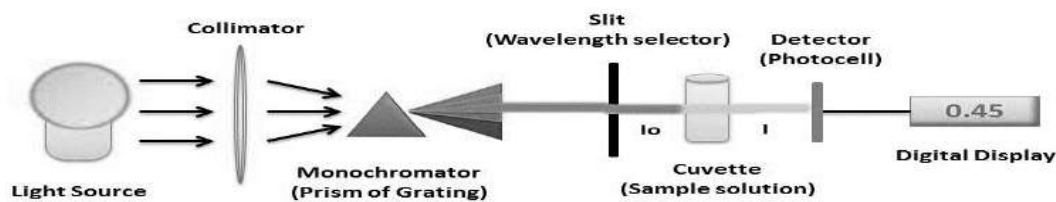
Basic Instrumentation of a Spectrophotometer
