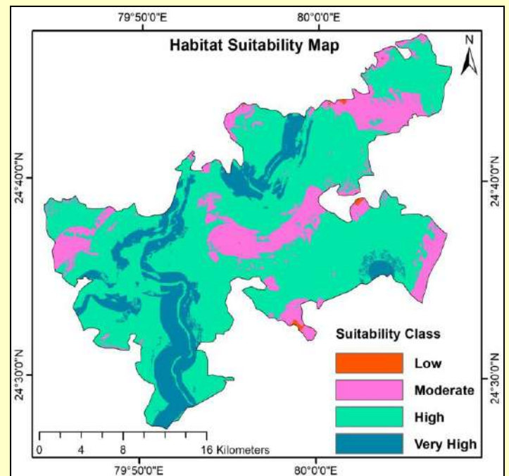
Habitat suitability map for Tiger at PTR
