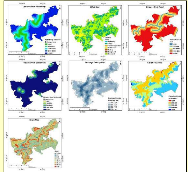
Assign parameter for habitat suitability
