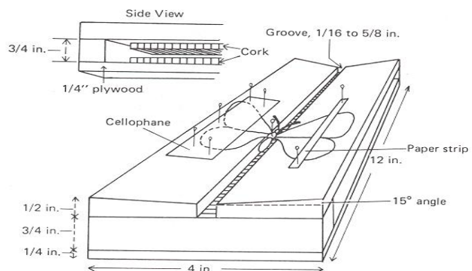
Spreading board used to spread insect wings
